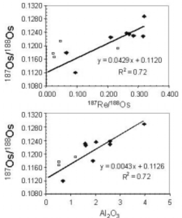
Fig. 1. ^{187}\text{Os}/^{188}\text{Os} versus \text{Al}_2\text{O}_3 and ^{187}\text{Re}/^{188}\text{Os} for xenoliths from Mojavia (filled diamonds) and the Colorado Plateau (open squares). Line is regressed through Cima data only.
