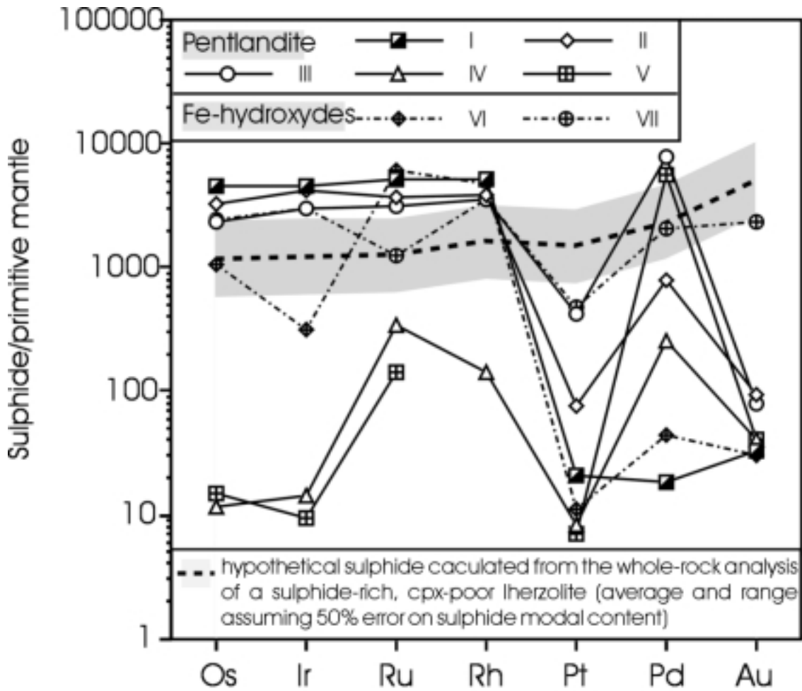
Fig.1: LAM-ICPMS analyses of sulphides.
